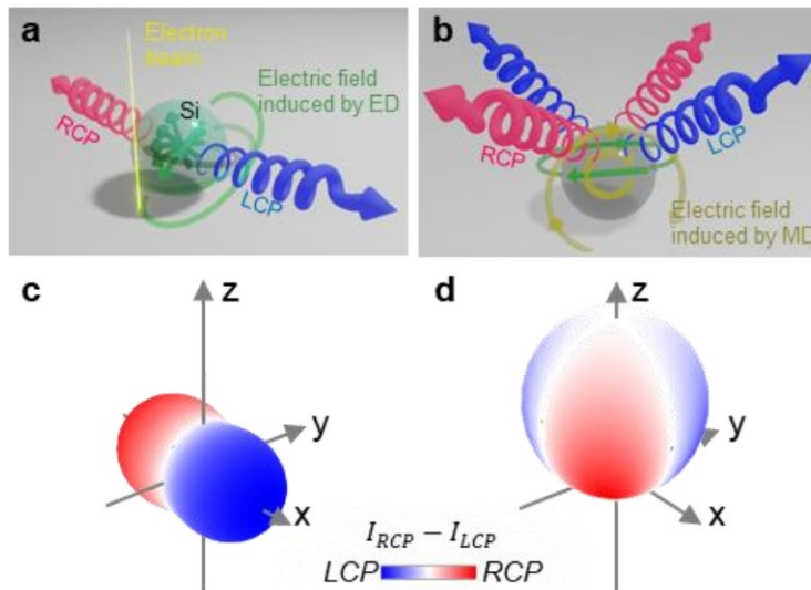
Figure 1. Two ways of generating CPL from a sphere
